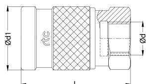
Free-Flow Coupling Kupplung ohne Ventil
